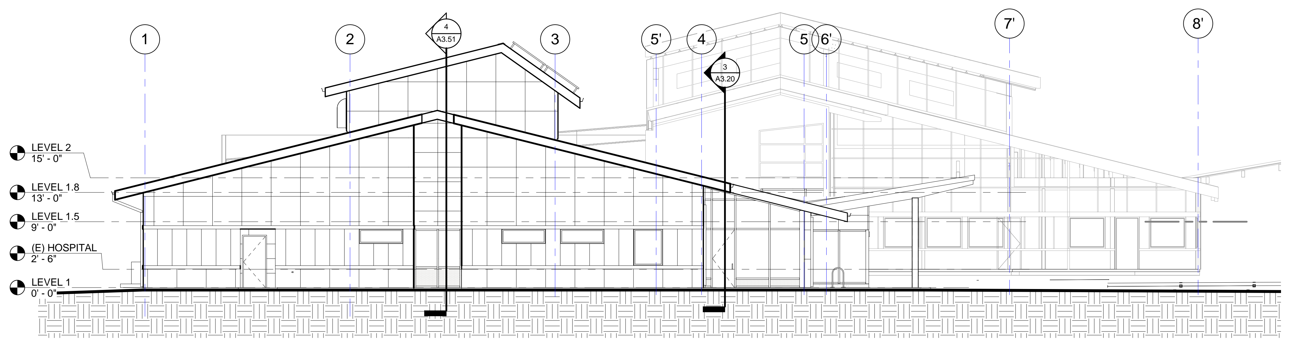
4 WEST 1/8" = 1'-0"
