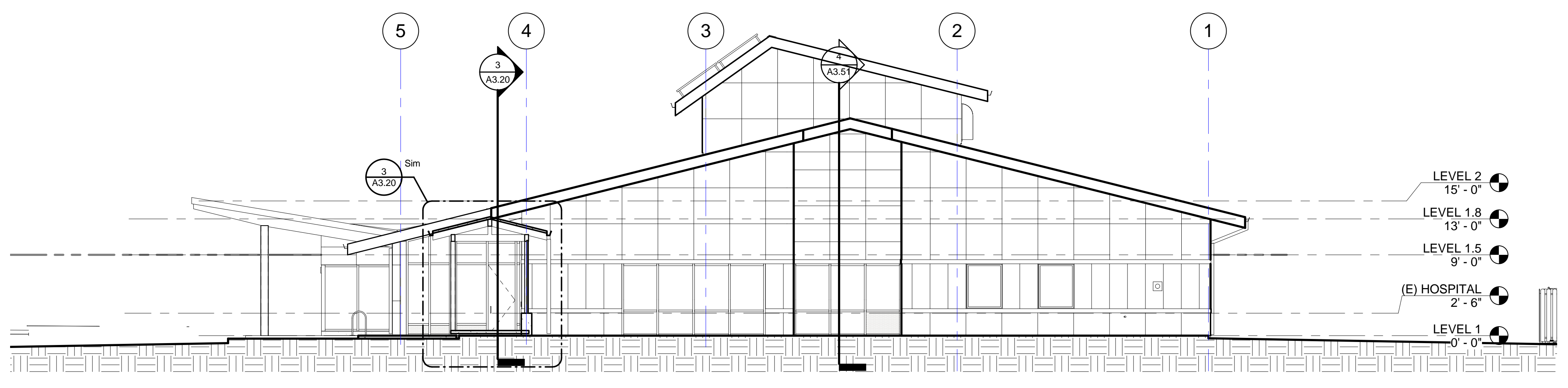
3 EAST 1/8" = 1'-0"
