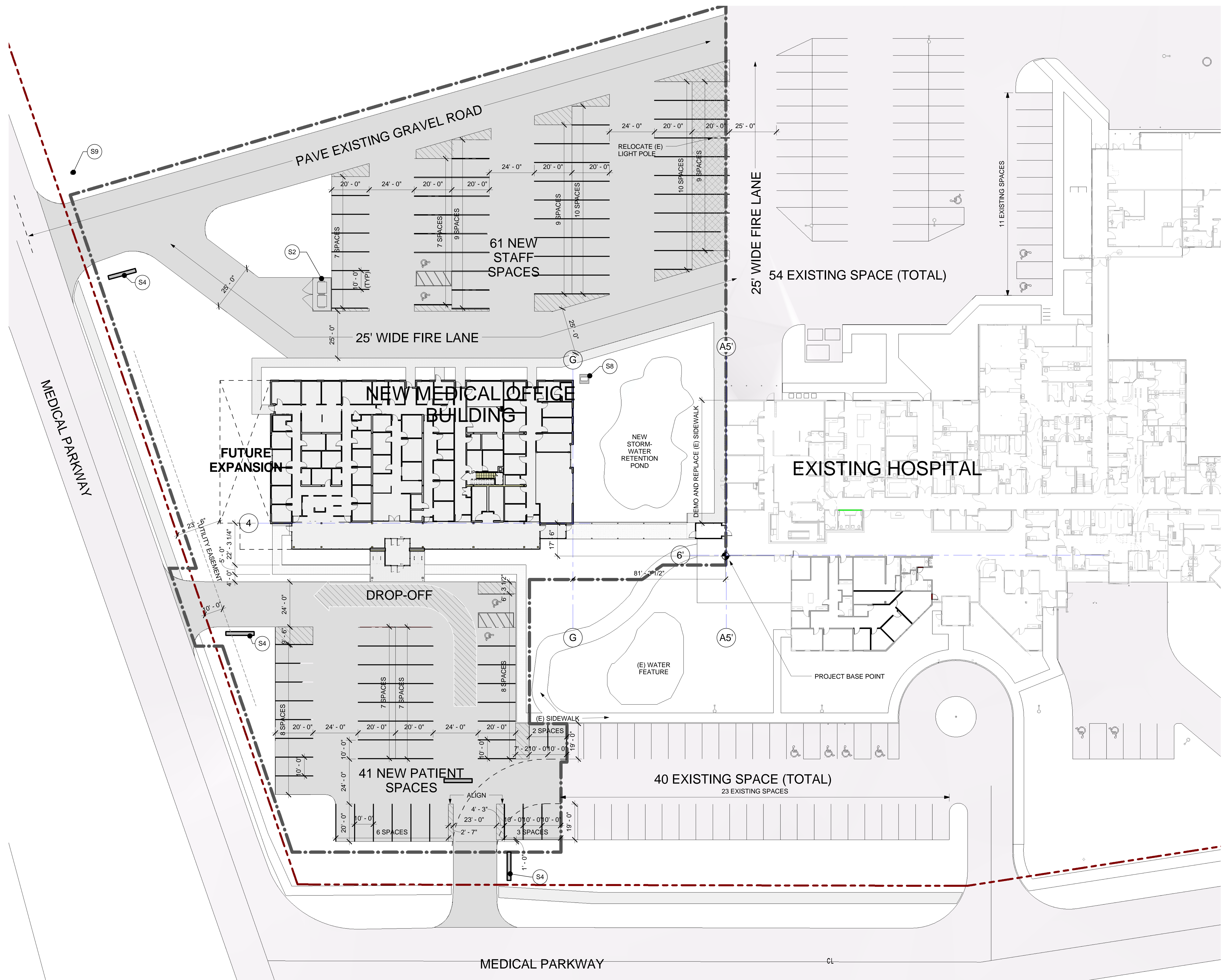
1 ARCHITECTURAL SITE PLAN 1" = 20'-0"
