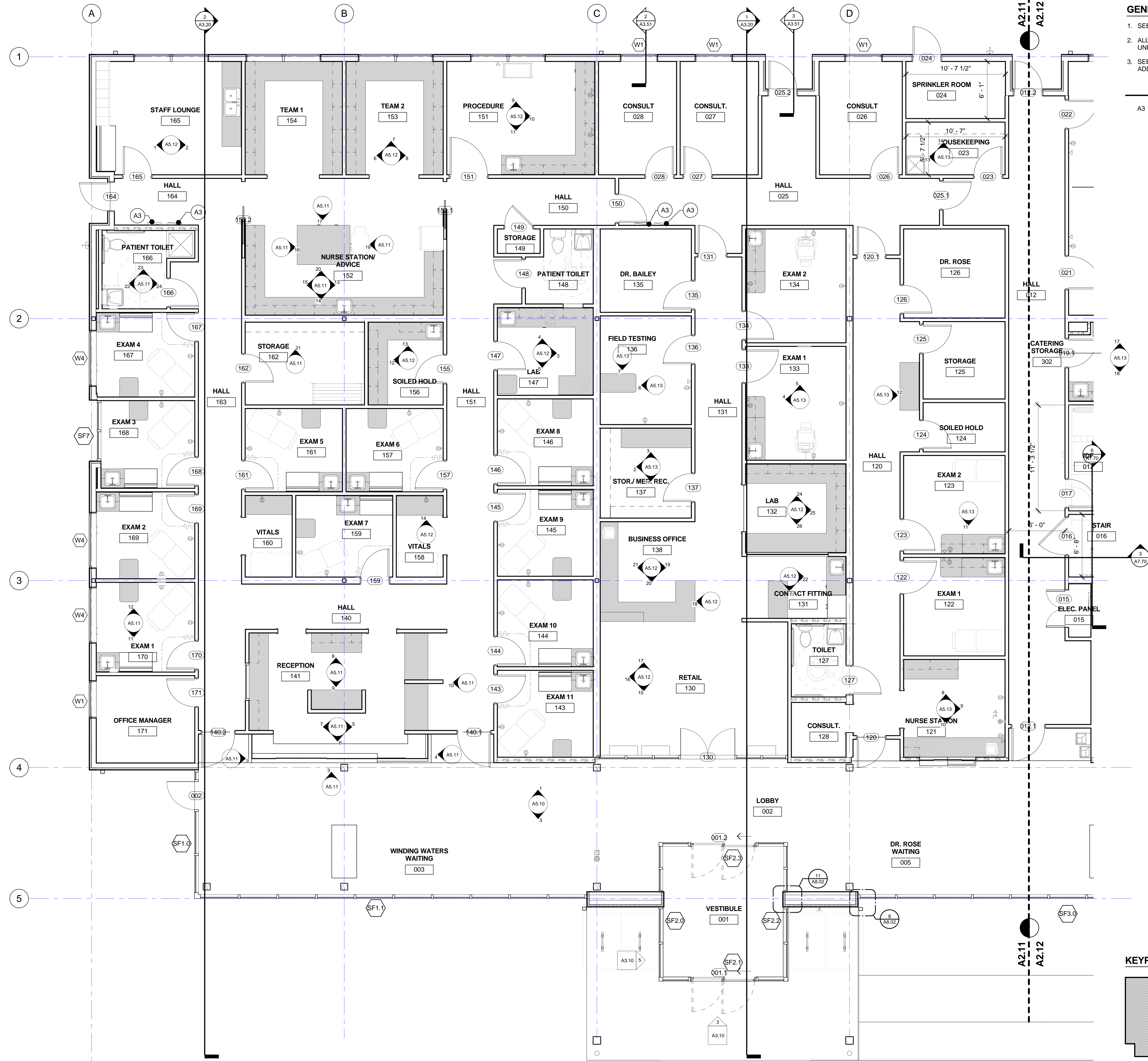
1 ENLARGED PLAN - LEVEL 1 WEST 1/4" = 1'-0"
